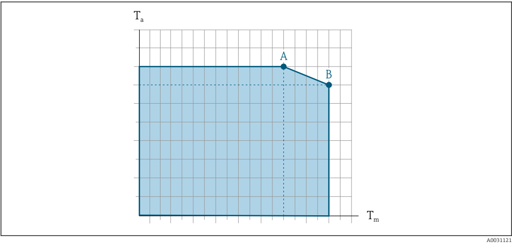
22 Exemplary representation, values in the table below. T a Ambient temperature T m Medium temperature A Maximum permitted medium temperature T m at T a max = 60 °C (140 °F); higher medium temperatures T m require a reduced ambient temperature T a B Maximum permitted ambient temperature T a for the maximum specified medium temperature T m of the sensor
