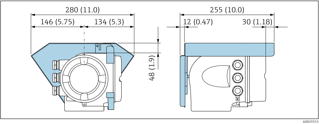
Protective cover
