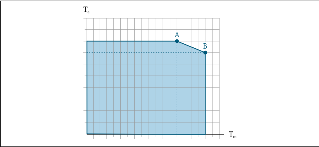
28 Exemplary representation, values in the table below. T_a Ambient temperature T_m Medium temperature A Maximum permitted medium temperature T_m at T_{a\max} = 60\text{ °C} (140 °F); higher medium temperatures T_m require a reduced ambient temperature T_a B Maximum permitted ambient temperature T_a for the maximum specified medium temperature T_m of the sensor
