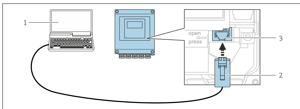
67 Connection via service interface (CDI-RJ45)
