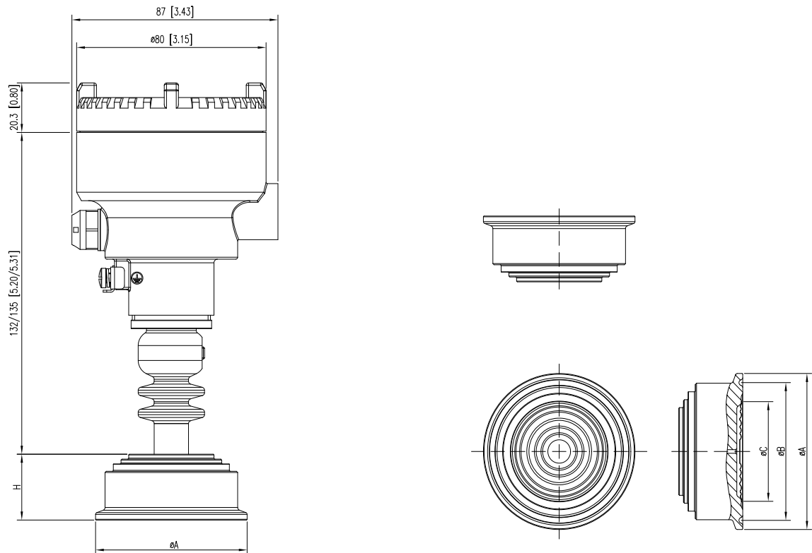
Figure 8 PXF100 with TRI CLAMP ISO 2852
