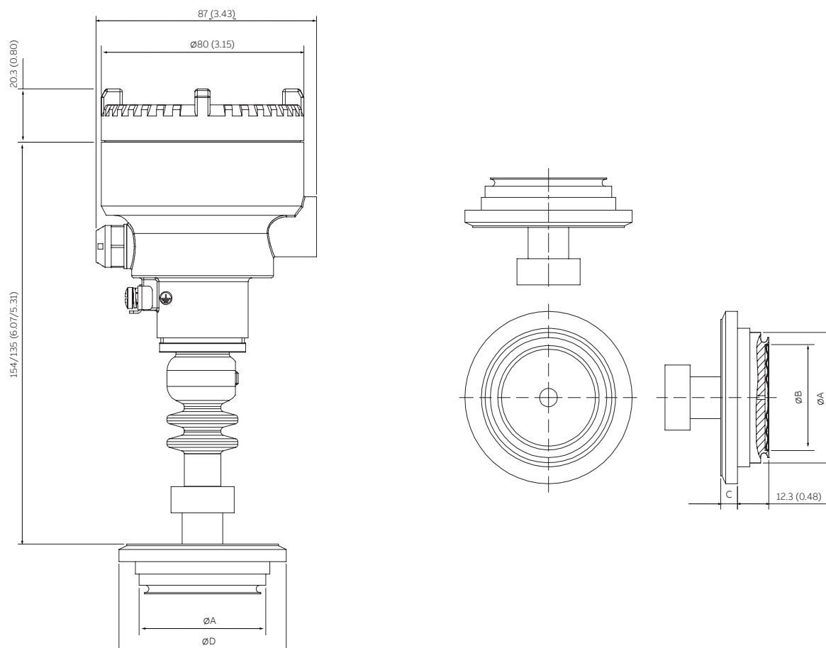
Figure 10 PXF100 with Varinline®
