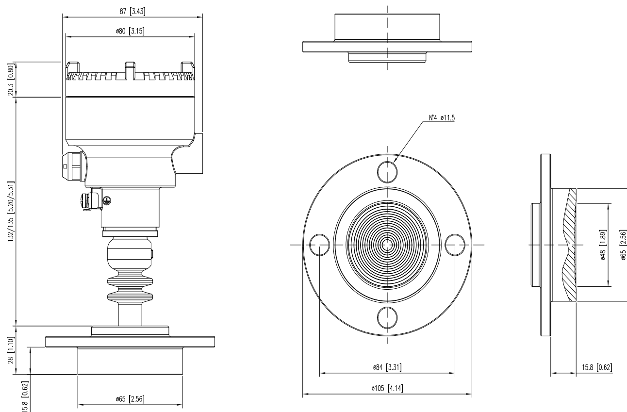
Figure 12 PXF100 with DRD
